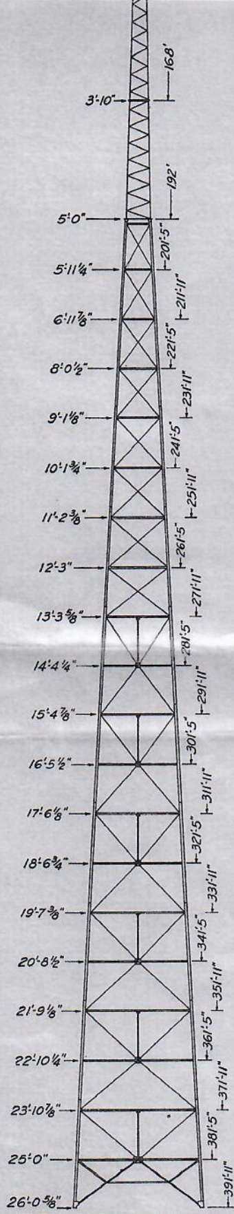
TRUSCON TRIANGULAR RADIO TOWER TYPE - C SELF-SUPPORTING MAXIMUM HEIGHT - 391 FEET TRUSCON STEEL COMPANY YOUNGSTOWN, OHIO.
